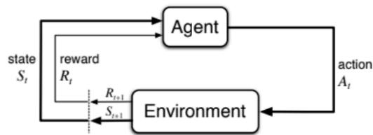
Gambar 2.1 Skema Reinforcement Learning (Sutton dan Barto, 2020)
