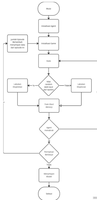
Gambar 3.2 Skema Deep Q Network
